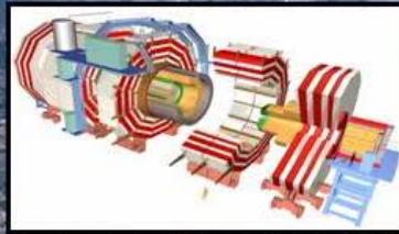
CMS
