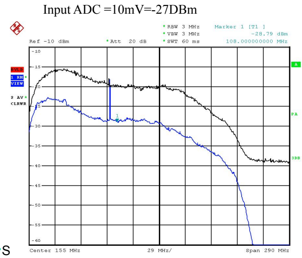
LNA+ Amplifier+ 50mcable + Mixer Gain (F)
