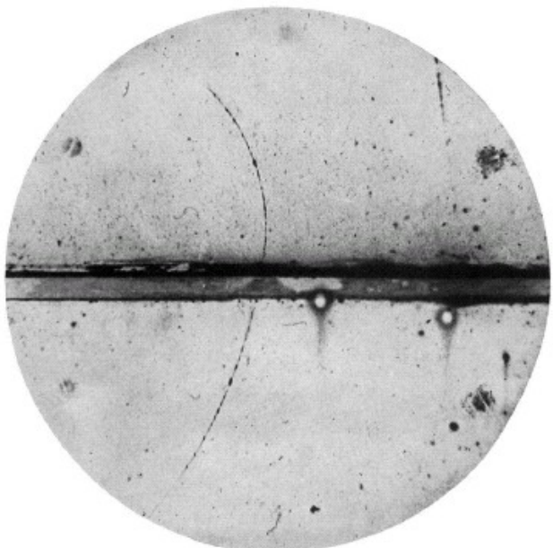
FIG. 1. A 65 million volt positron ( H\rho=2.1 \times 10^6 gauss-cm) passing through a 6 mm lead plate and emerging as a 23 million volt positron ( H\rho=7.5 \times 10^6 gauss-cm). The length of this latter path is at least ten times greater than the possible length of a proton path of this curvature.
