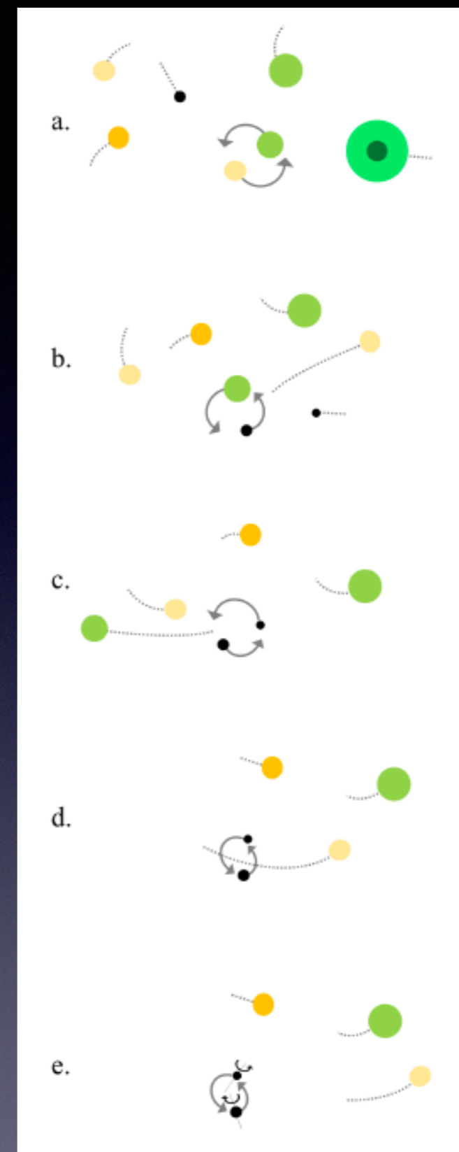
Formation scenarii: isolated (CE), CHE, dynamical (Mandel & Farmer 2018)
