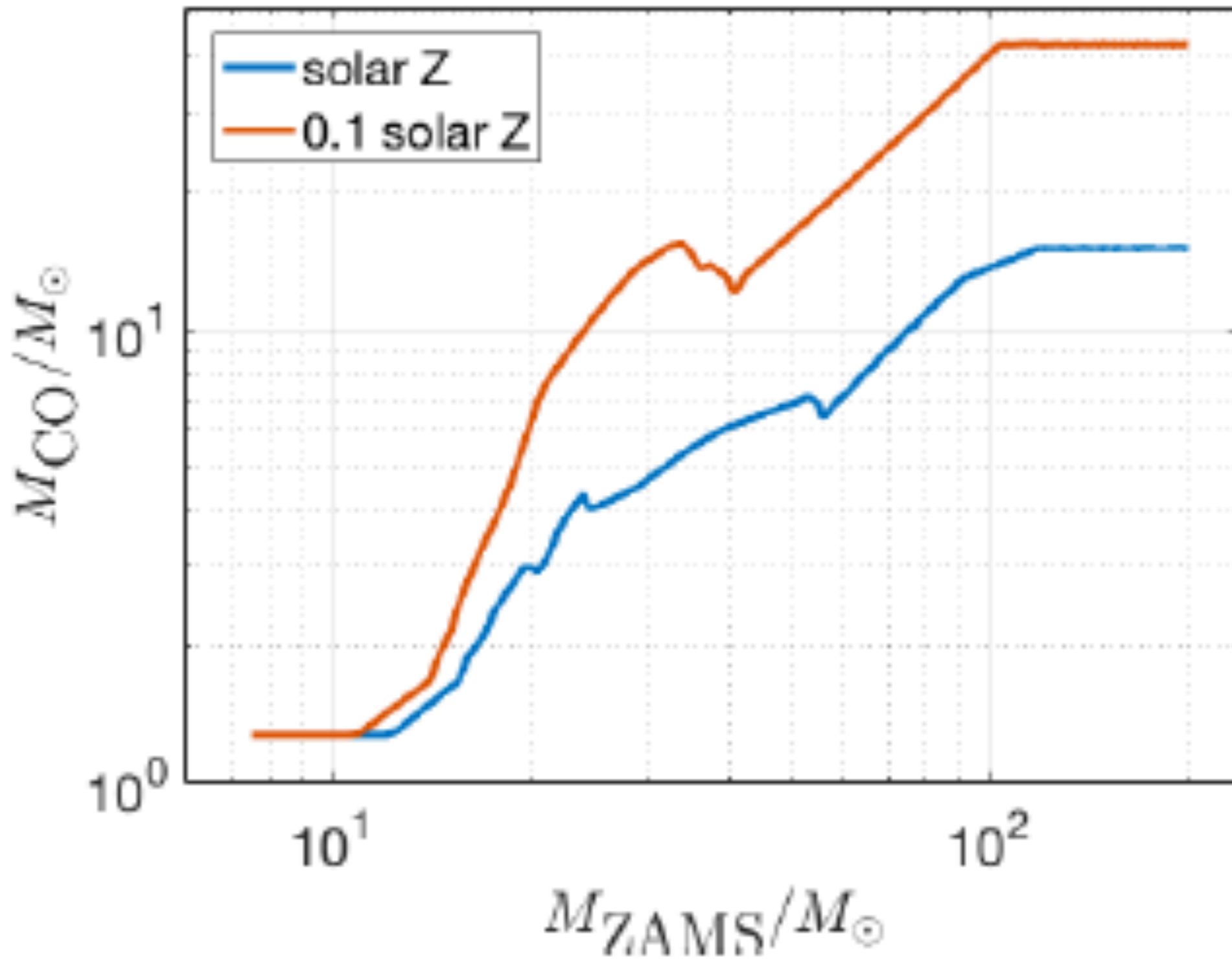
Mass of remnant compact object (Stevenson et al 2017)
