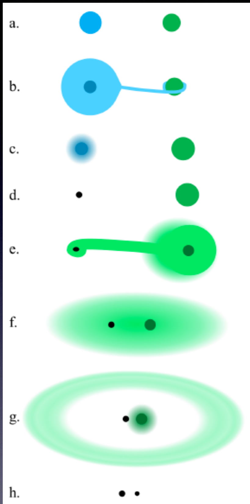
Formation scenarii: isolated (CE), CHE, dynamical (Mandel & Farmer 2018)
