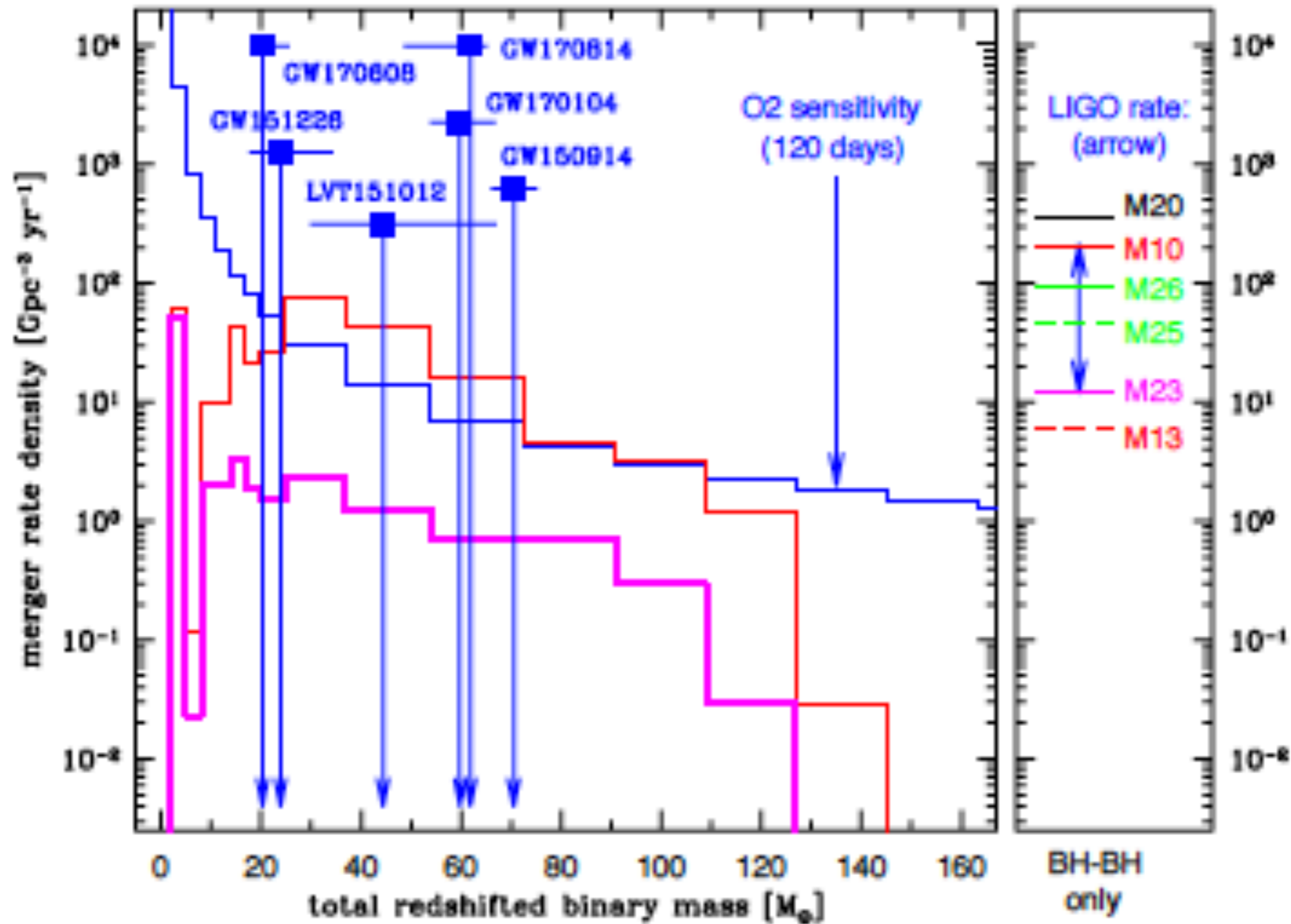
Merger rate density (Barack et al 2018)
