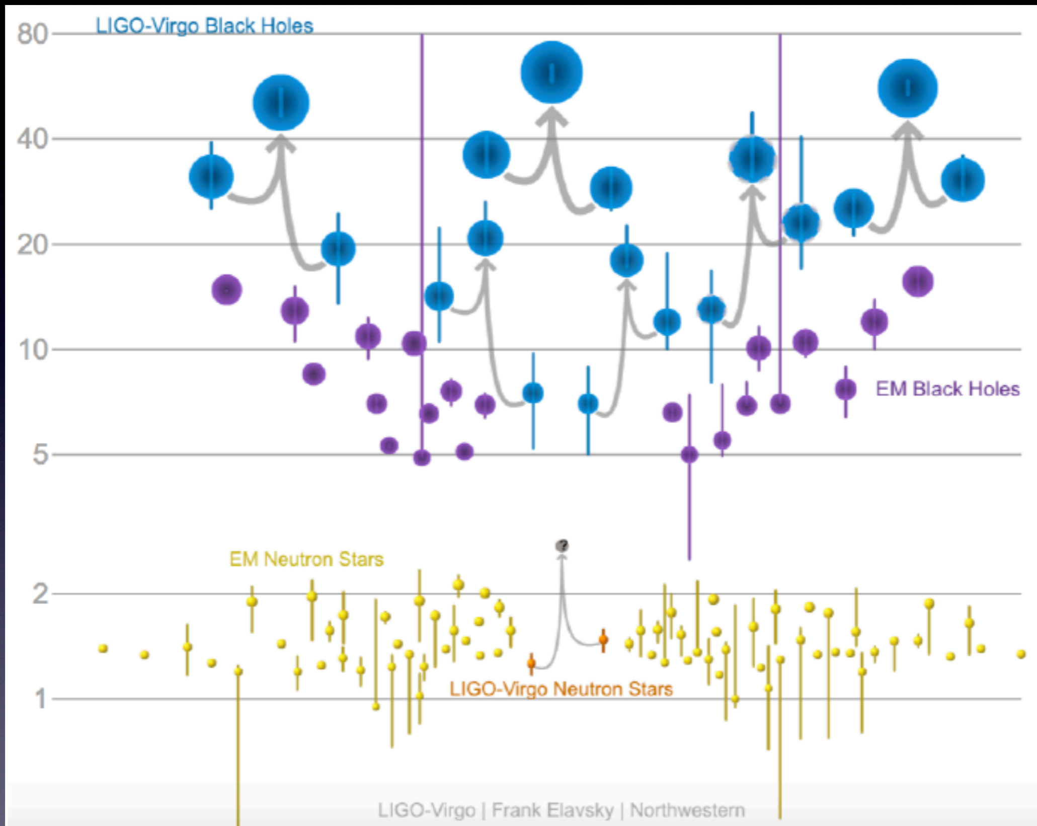
Mass spectrum (NS, BH) (LIGO-Virgo collaboration)
