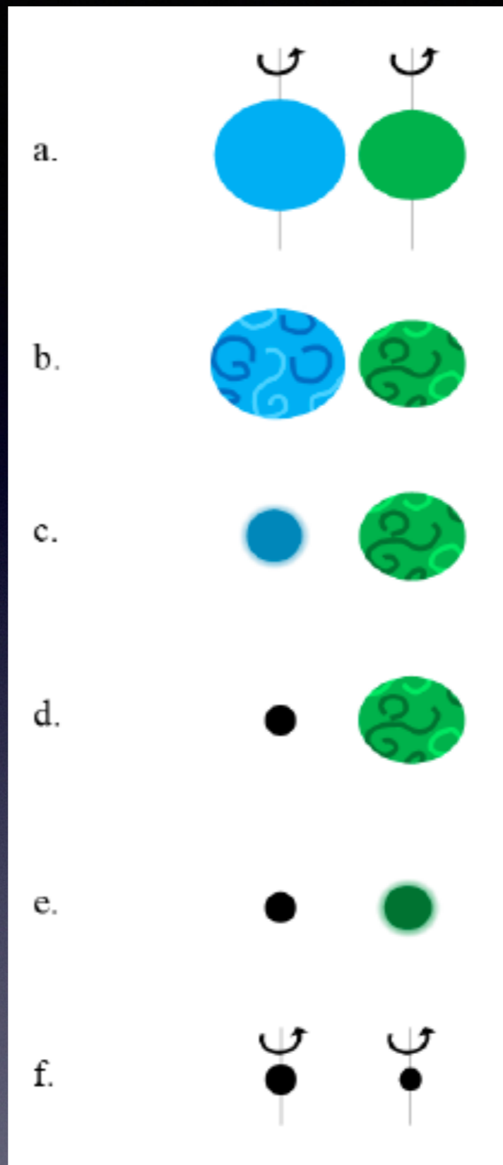
Formation scenarii: isolated (CE), CHE, dynamical (Mandel & Farmer 2018)
